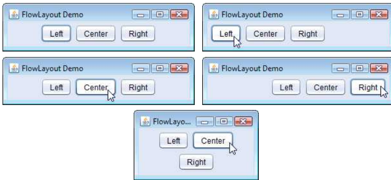
Fig. 12.40 | Testing FlowLayoutFrame.
